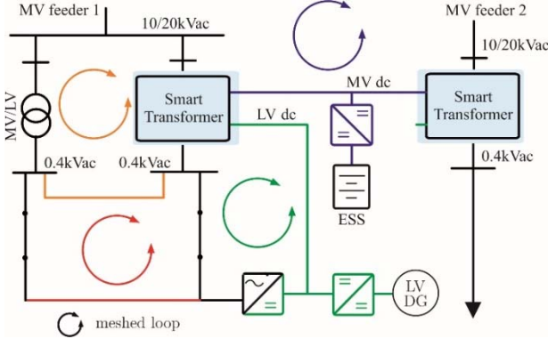
Fig. 3 ST-enabled configurations of a meshed hybrid distribution grid.
